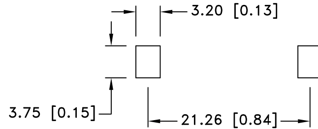
PCB LAYOUT
