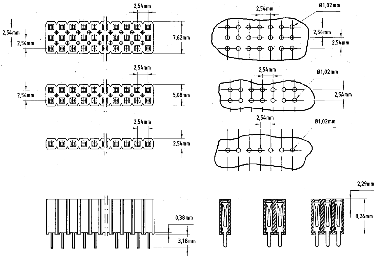
Recommended Mounting Hole Patterns
