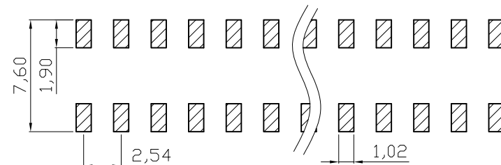
Recommended PCB Layout(Top Side) ( PCB BOARD TOLERANCE±0.05)
