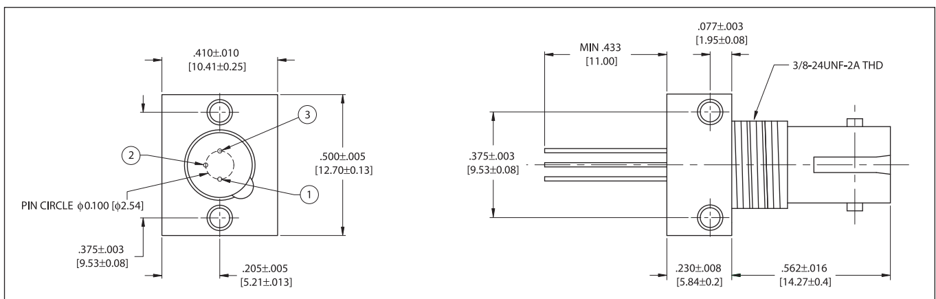
ST Receptacles Package
