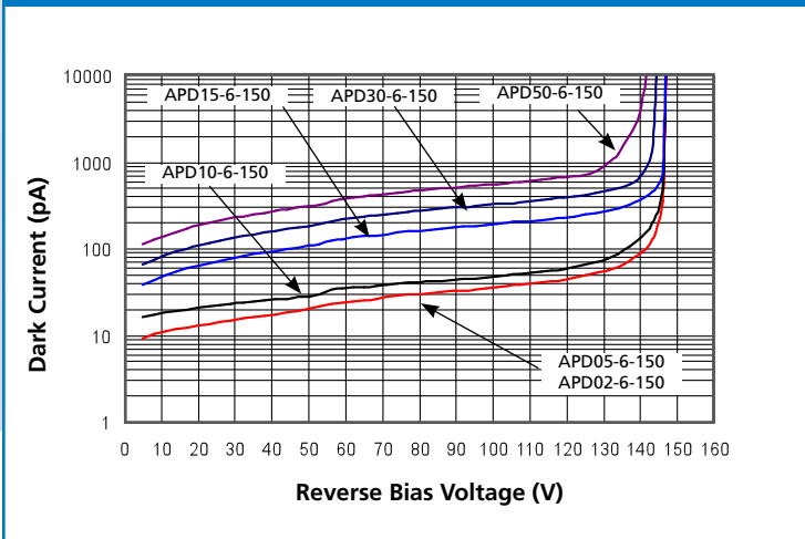
Typ. Dark Current vs. Reverse Bias ( T_A = 23^\circ\text{C} )
