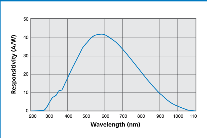
Typ. Spectral Response ( T_A = 23^\circ\text{C} , M = 100 )
