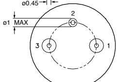
Pin Circle Dia = 7.5
