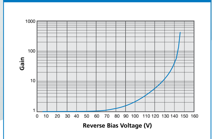
Typ. Gain vs. Reverse Bias ( T_A = 23^\circ\text{C} , 630 nm)
