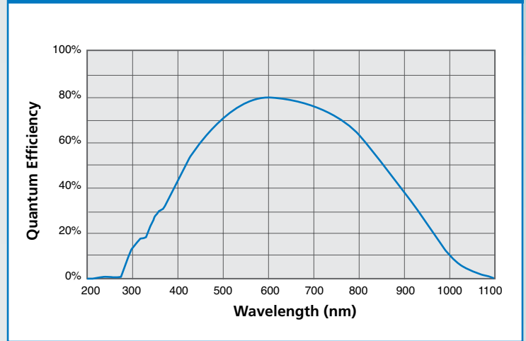
Typ. Quantum Efficiency vs. Wavelength ( T_A = 23^\circ\text{C} )
