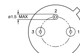
Pin Circle Dia = 5.08
