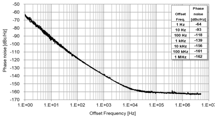
(15) fo = 48 MHz, T_use = +25 °C, n = 5 pcs
