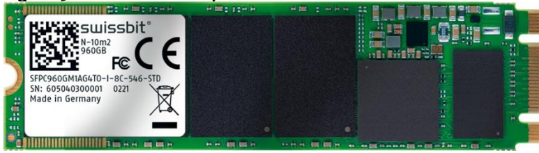
Figure 5: N-10m2 2280 top view
