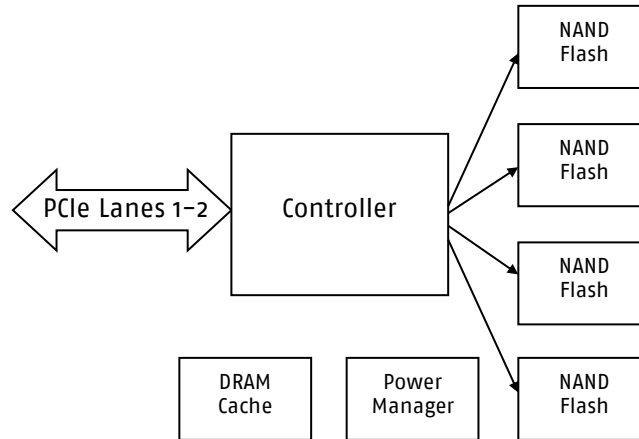
Figure 1: N-10m2 2280 Functional Block Diagram
