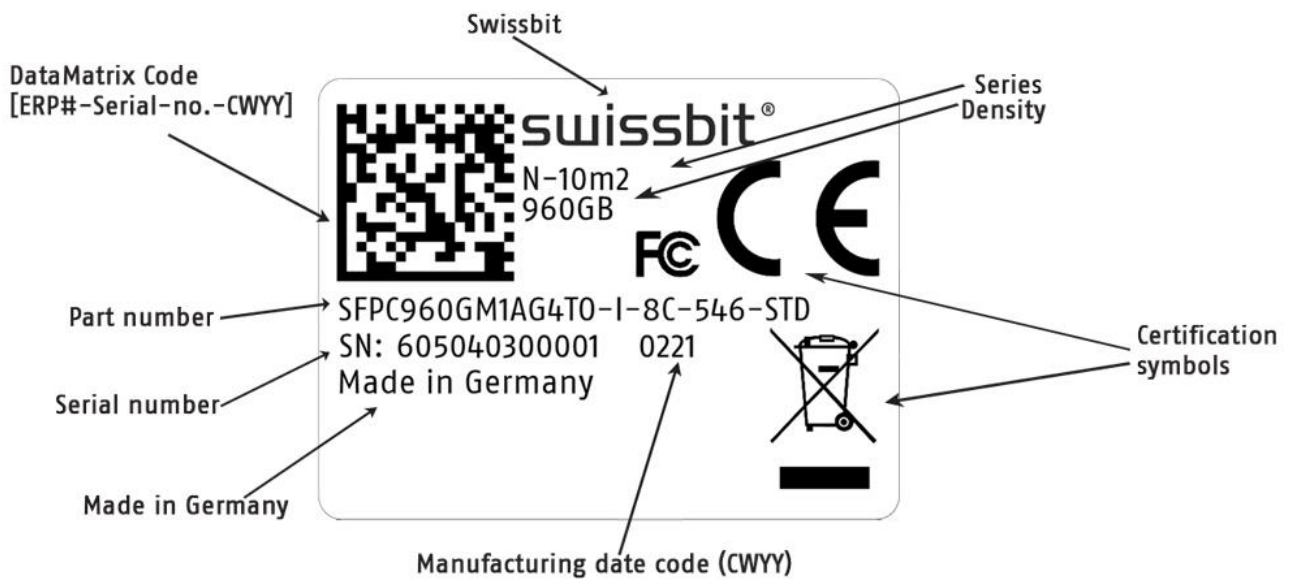
Figure 6: N-10m2 2280 label details
