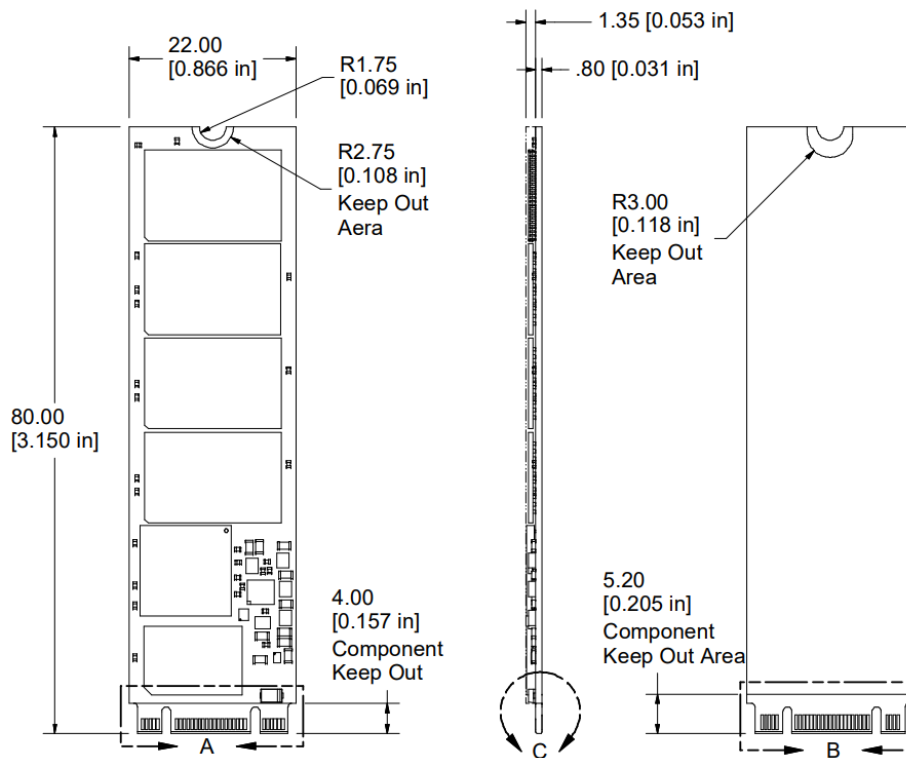
Figure 3: N-10m2 2280 dimensions in mm [in]
