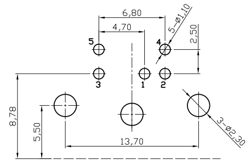
RECOMMENDED P.C.B. PATTERN LAYOUT TOP VIEW (TOLERANCE: ±0.05)
