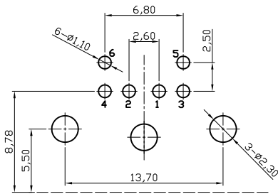
RECOMMENDED P.C.B. PATTERN LAYOUT TOP VIEW (TOLERANCE: ±0,05)
