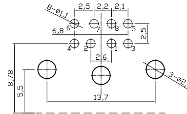
RECOMMENDED P.C.B. PATTERN LAYOUT TOP VIEW (TOLERANCE: ±0.05)
