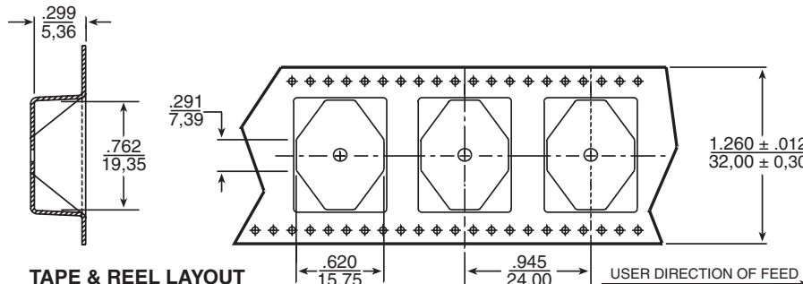
TAPE & REEL LAYOUT
