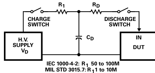
ELECTROSTATIC DISCHARGE TEST
