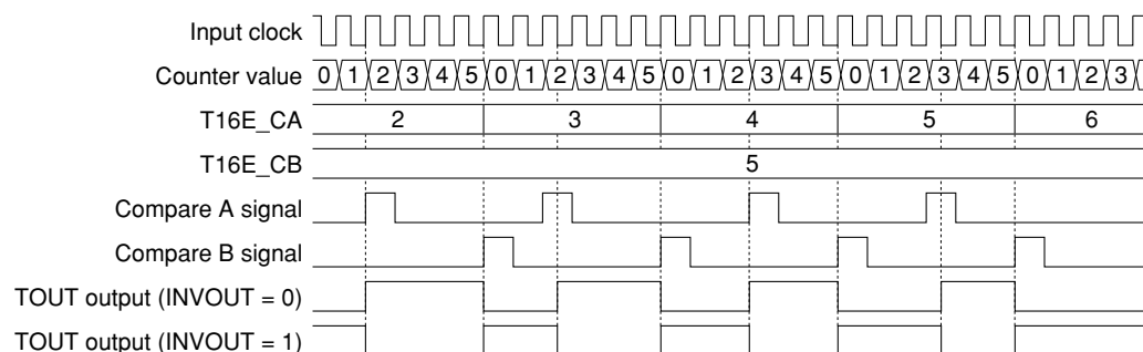
Figure 13.6.3 Clock Output in Fine Mode
