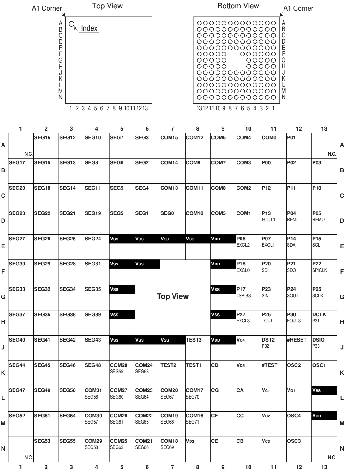
Figure 1.3.1.3 Pin Arrangement (VFBGA7H-161)
