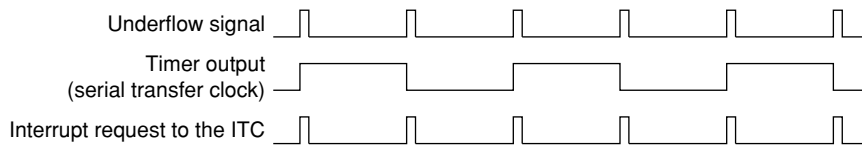
Figure 12.7.1 Timer Output Clock
