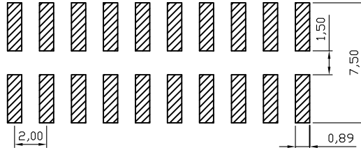
Recommended P.C.B Layout(Top Side) (PCB BOARD TOLERANCE±0.05)
