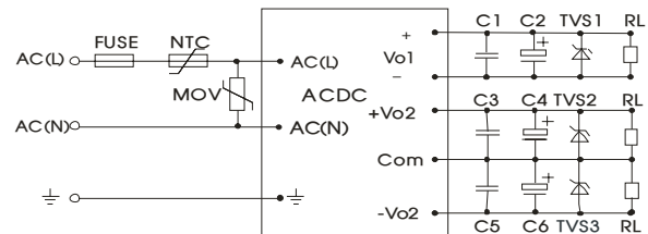
Fig. 4: LHxx-10Cxx (Triple Output) series typical application circuit
