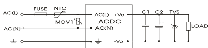
Fig. 1: Typical application circuit
