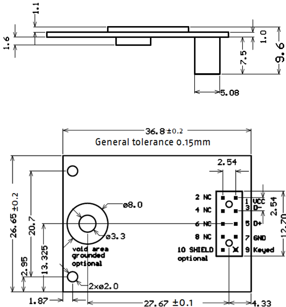
Figure 2: Mechanical Dimensions for 2.54mm connector (standard)
