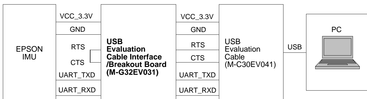
Fig1. Block Diagram
